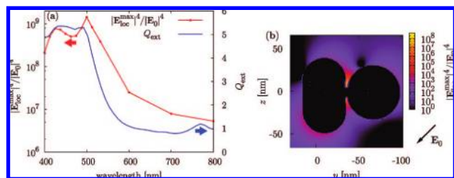
Figure 3. Optical properties of the SMSERS active structure in Figure 2a obtained from 3D calculations using DDA. The structure is approximated as a T-shaped dimer consisting of a sphere and a hemispherically capped rod that just touch (0 nm separation). (a) Extinction efficiency (blue line) and maximum SERS enhancement E_{EM} , calculated as |E_{loc}|^4/|E_0|^4 , (red line) for each wavelength. (b) Contour plot of E_{EM} at the plane x = -4 nm, where the maximum value of E_{EM} = 3.9 \times 10^8 at 532 nm is observed. For reference the plane x = 0 is defined as where two Ag nanocrystals touch, indicating the hot spot is localized at the cusp between the particles.
